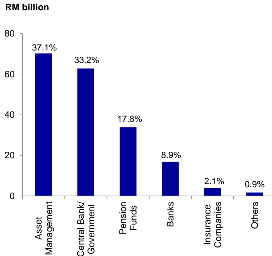
Distribution of Non-resident Holdings of Government Bonds as at end-September'20
